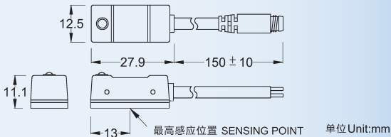
XYC-21P / XYC-21P-QD XYC-21N / XYC-21N-QD
