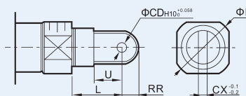
单U型钩 Single U-type
