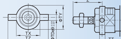
耳轴 Bearing
