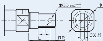
双U型钩 Double U-type
