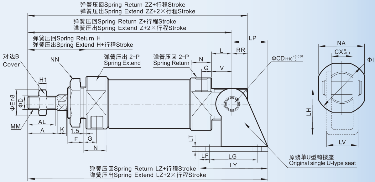
原装单U型钩接座 Original Single U-type Seat
