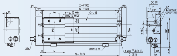
C□Y1S15.20.32.40
